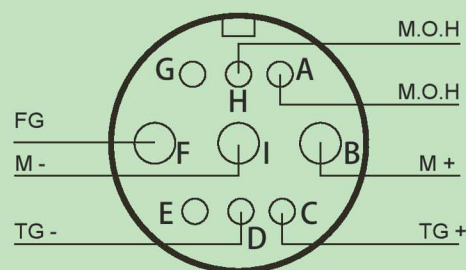
MS conect #3102A 20-18P
